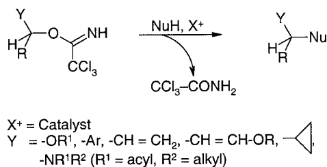
Scheme 1. Acid-catalyzed alkylation of nucleophiles with O -alkyl trichloroacetimidate derivatives
