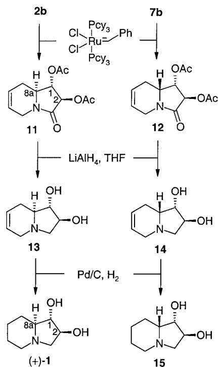
Scheme 7. Synthesis of target molecule (+)- 1 and its epimer 15
