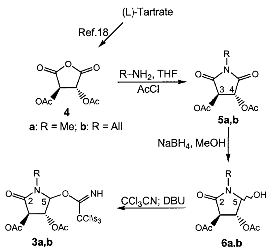
Scheme 4. Synthesis of O -(2-oxopyrrolidin-5-yl)trichloroacetimidates 3a,b
