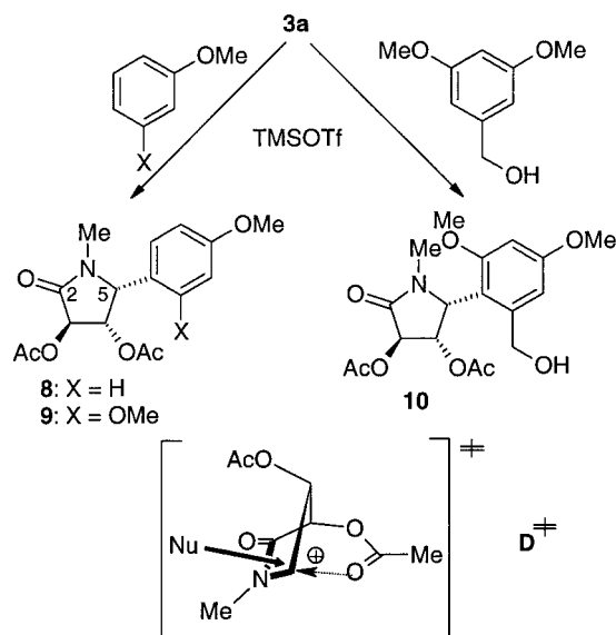
Scheme 6. Arylation of 3b with electron-rich aromatic compounds
