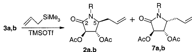
Scheme 5. Allylation of 3a,b with allyltrimethylsilane
